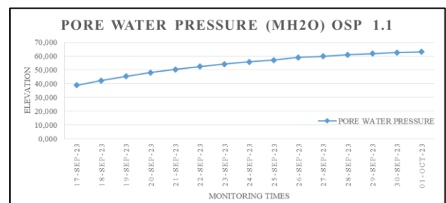
Figure 6. Graph of pore water pressure against Casagrande piezometer measurement time
